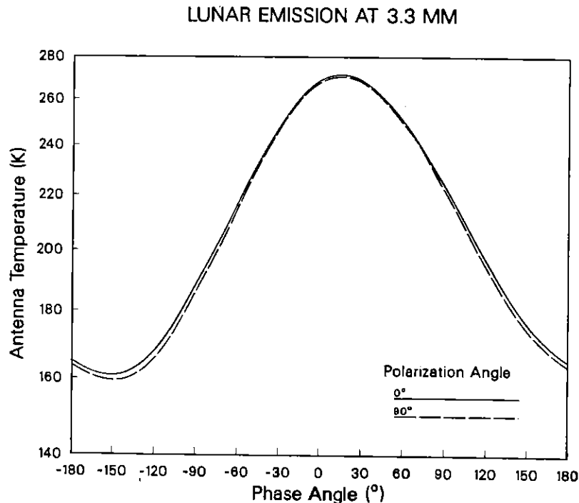
Fig. 8. - Full disk equivalent brightness temperature of the moon versus phase angle. Phase angle for the Brazilian flight was -134^\circ .
