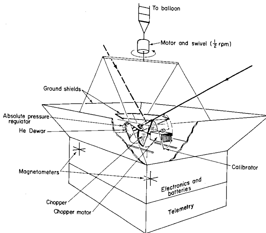
Fig. 1. - Gondola and instrumentation.
