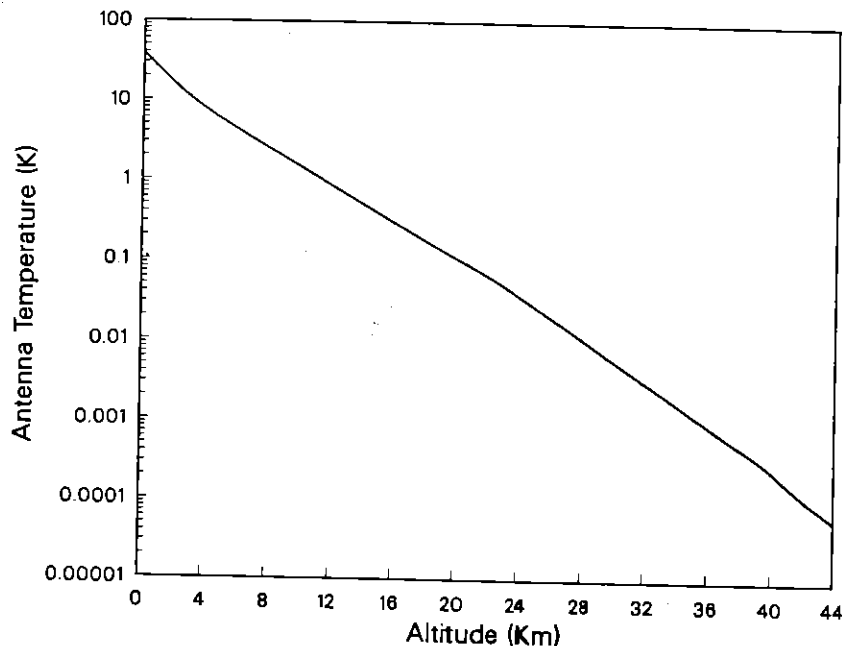
Fig. 5. - Calculated vertical atmospheric emission versus altitude.
