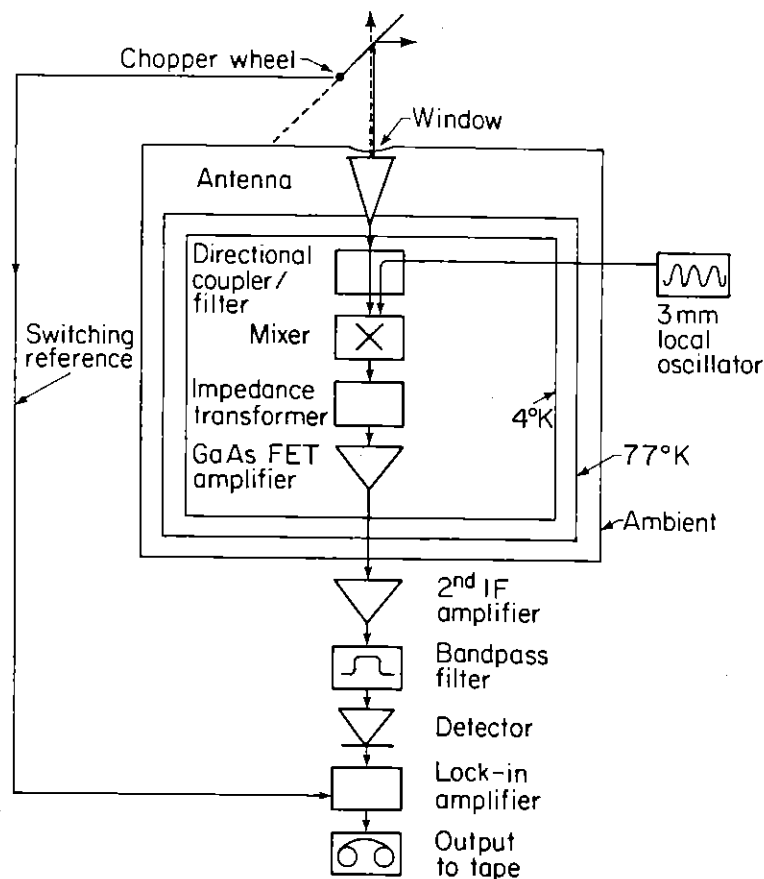
Fig. 2. - Schematic of 3.3 mm radiometer.
