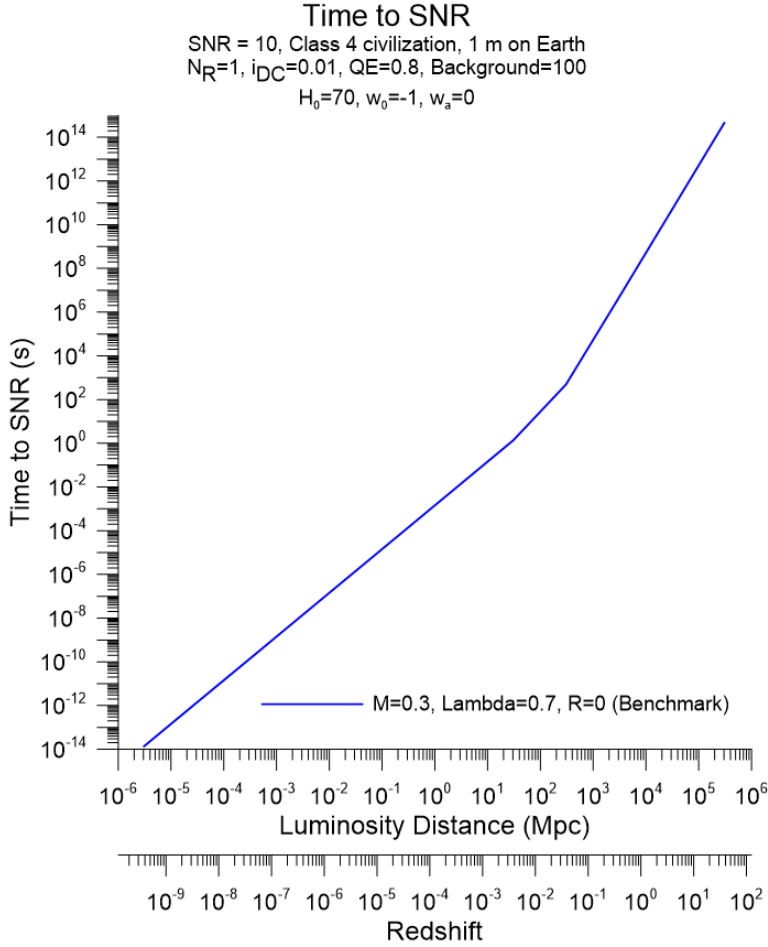
Figure 26 – Time to SNR vs luminosity distance and redshift. Here the SNR is set to 10 for a 1m ground based wide field survey that observes the full sky all the time with an integration time of 1000 s. The transmitting civilization is Class 4. A benchmark or concordance model is used for the cosmological relationship between luminosity distance and redshift.
