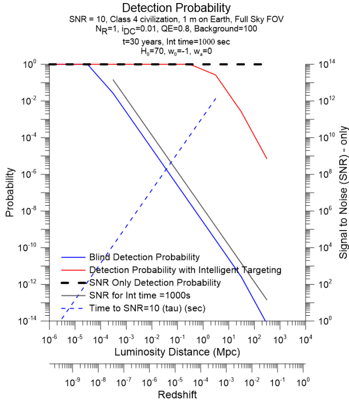
Figure 27 – Probability of detection vs luminosity distance and redshift for a modest 1m ground based wide field survey that observes the full sky all the time with an integration time of 1000 s per image. The transmitting civilization is Class 4. Three types of detection probability are shown. One is based only on achieving the SNR (10 here) for a single integration time and assumes the Earth based system views the transmitter beam. The second (blue) is a blind survey of a SINGLE civilization that randomly (or uniformly) scans the sky during a 30 year Earth observing campaign. As can be seen the blind survey could easily detect the civilization if it were pointing at the Earth. The third (red) is computed assuming “intelligent targeting” is used where known stars “habitable zones” are targeted, using the “gain factor” discussed, rather than simply a uniform scan. Note that in this case the probability of detection increases dramatically. The SNR (dark grey) for integration time = 1000 s is also shown and uses the right-hand Y axis. The integration time to SNR=10 (blue dashed) is also shown – use left-hand Y axis. A benchmark or concordance model is used for the cosmological relationship between luminosity distance and redshift.
