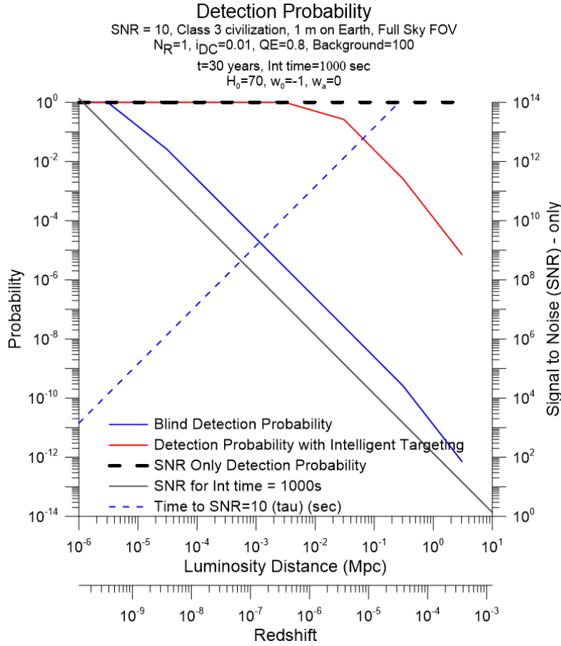
Figure 28 – Probability of detection vs luminosity distance and redshift for a modest 1m ground based wide field survey that observes the full sky all the time with an integration time of 1000 s per image. The transmitting civilization is Class 3. Three types of detection probability are shown. One is based only on achieving the SNR (10 here) for a single integration time and assumes the Earth based system views the transmitter beam. The second (blue) is a blind survey of a SINGLE civilization that randomly (or uniformly) scans the sky during a 30 year Earth observing campaign. As can be seen the blind survey could easily detect the civilization if it were pointing at the Earth. The third (red) is computed assuming “intelligent targeting” is used where known stars “habitable zones” are targeting, using the “gain factor” discussed, rather than simply a uniform scan. Note that in this case the probability of detection increases dramatically and even a class 3 civilization can be seen throughout our galaxy in an intelligently targeted transmitting survey. The SNR (dark grey) for integration time = 1000 s is also shown and uses the right-hand Y axis. The integration time to SNR=10 (blue dashed) is also shown – use left-hand Y axis.
