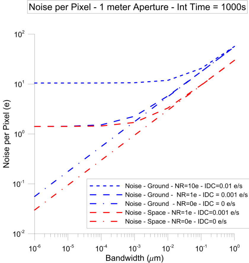
Figure 21 – Noise per pixel vs filter bandwidth for several hypothetical wide field cases. Includes detector noise is given as well as background noise. For small filter bandwidths the noise is detector noise limited while for large bandwidth the noise is background limited. At very large bandwidth the noise converges and is proportional to \beta^{1/2} where \beta is the filter bandwidth. For a space mission the measurements are limited by zodiacal light and detector noise, assuming the optics are cooled sufficiently (for the IR cases) as to not dominate. In general a space mission will use diffraction limited optics and there will be no atmospheric “seeing issues”. For the ground based cases we assume a wide field system and we assume adaptive optics cannot be used over the wide FOV. We also show a noiseless detector case for reference which could be realized for photons counting systems such as superconducting MKIDs (Microwave Kinetic Inductor Detector) or possible advanced cooled APD (Avalanche Photo Diode) arrays. Neither is currently available in the large formats ideally needed. For the ground case we assume the atmospheric transmission is 0.5, the pixel size is 0.5'' , the seeing is 1'' , the total telescope optical efficiency is 0.5, the detector QE = 0.5 and the atmospheric and extraterrestrial background is 100 \gamma/s\text{-m}^2\text{-}\mu\text{m}\text{-sq-arcsec} . Note that depending on the wavelength and the sky conditions the background could be significantly larger especially in the presence of OH lines in systems with low resolving power (wider filter bandwidth). For the space based case we assume the system is diffraction limited, the total telescope optical efficiency is 0.7, the detector QE = 0.8 and the extraterrestrial background is 10 \gamma/s\text{-m}^2\text{-}\mu\text{m}\text{-sq-arcsec} and that the optics are sufficiently cooled. The primary advantage of space is the lack of atmospheric emission, particularly of OH lines in J and H bands as well as the ability to cool the optics for K band and beyond.
