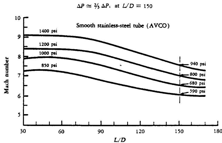
FIG. 38—Shock-tube Attenuation Data at High Overpressure
