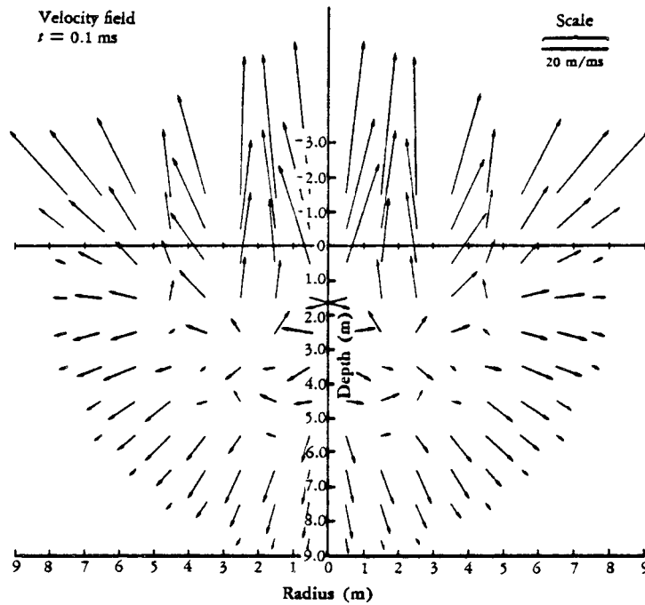
FIG. 15—Particle Velocities from Surface Burst ( t = 0.1 ms)
