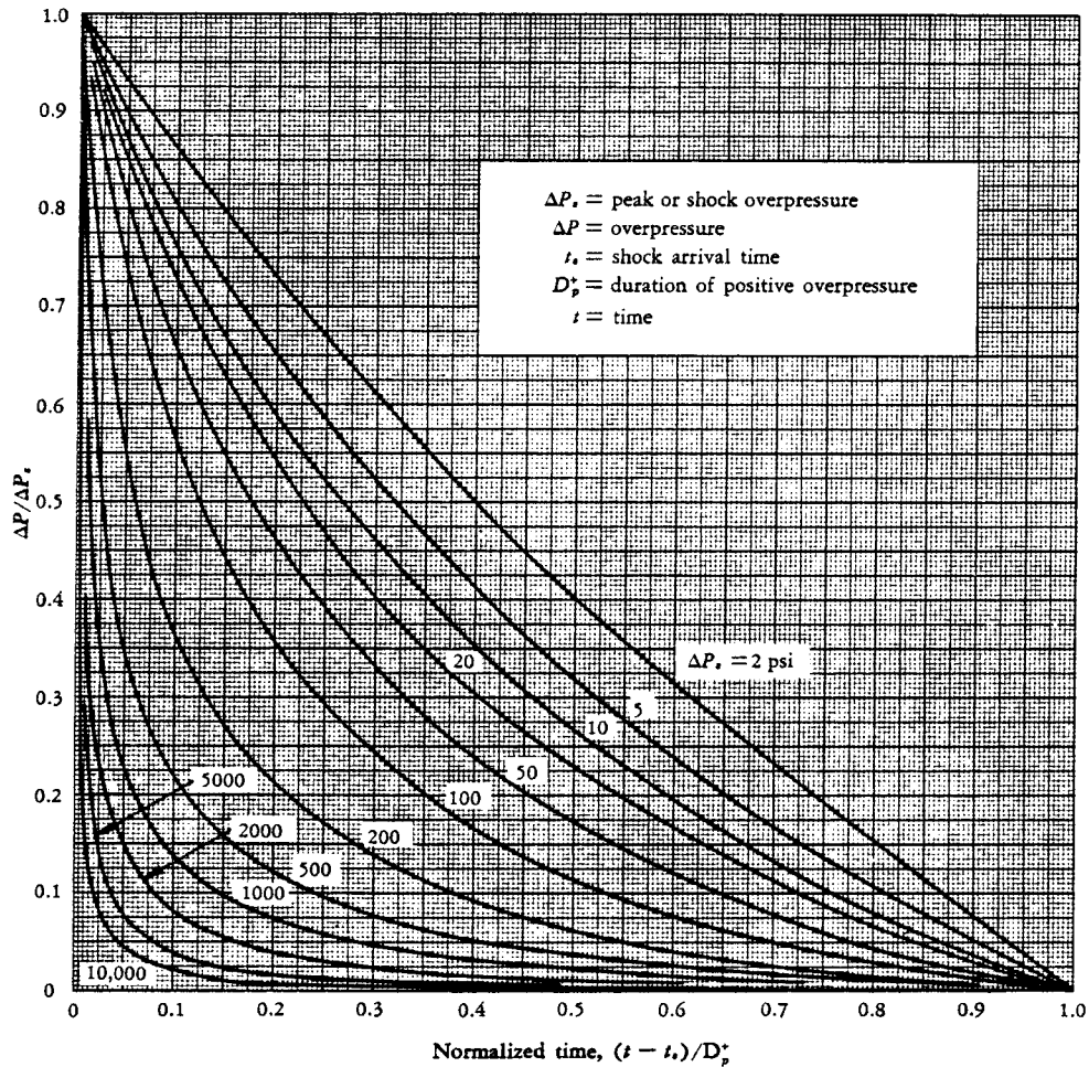
FIG. 26—Form Factors for Overpressures from Nuclear Explosions
