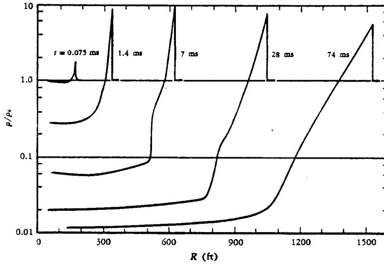
FIG. 3—Fireball Density versus Radius at Early Times in the Fireball History (1-MT Surface Burst)
