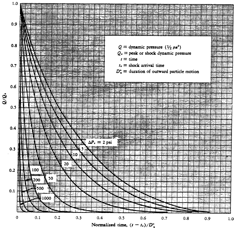
FIG. 27—Form Factors for Dynamic Pressures from Nuclear Explosions
