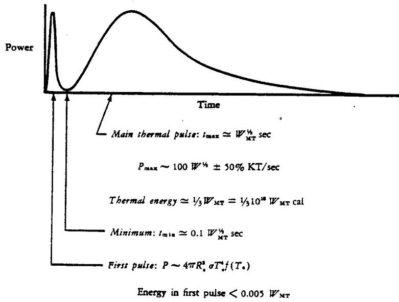
FIG. 6—Thermal Radiation Rate
