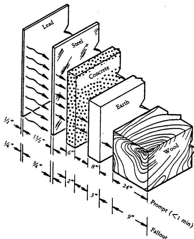
FIG. 10—Half-thickness for Gamma-ray Attenuation
