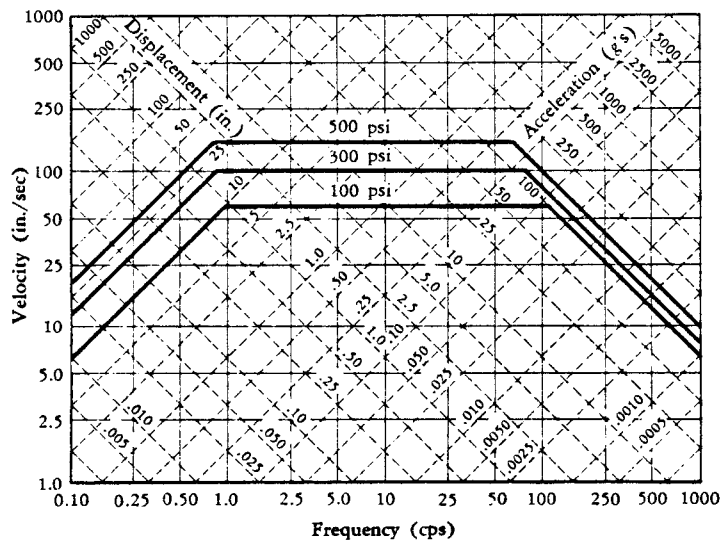
FIG. 45—Vertical Shock Spectra
