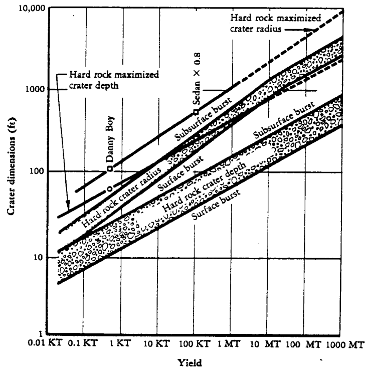
FIG. 12—Crater Scaling
