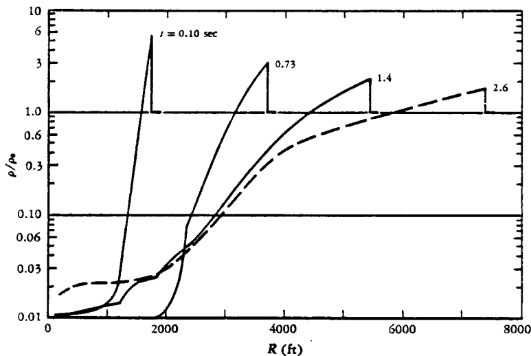
FIG. 46—Late Fireball Densities (1-MT Surface Burst)
