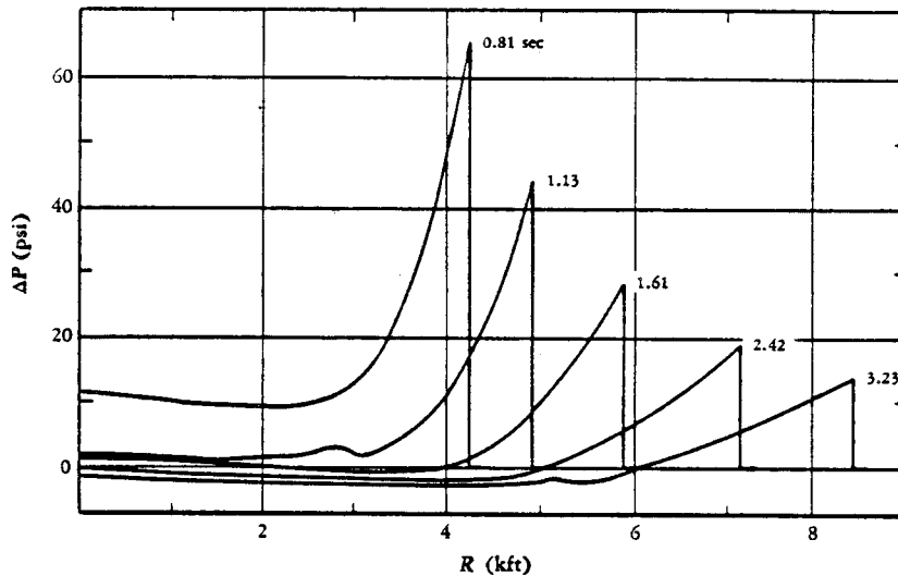
FIG. 22—Overpressure versus Radius (1-MT Surface Burst)
