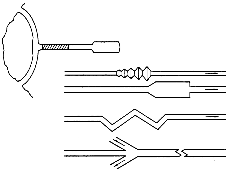
FIG. 40—Shock-attenuation Schemes
