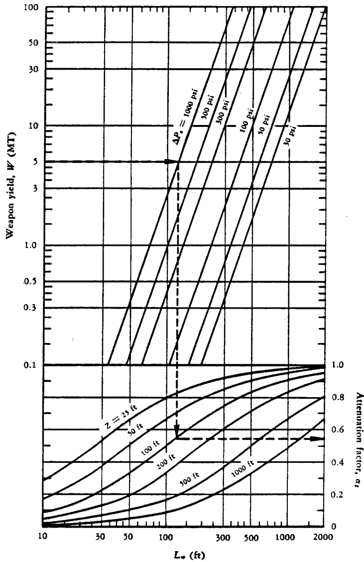
FIG. 44—Geometric Attenuation with Depth
