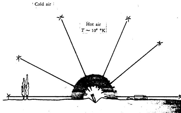
FIG. 1—Initial Fireball Growth
