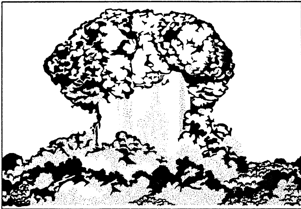
FIG. 47—Late Fireball Turbulence
