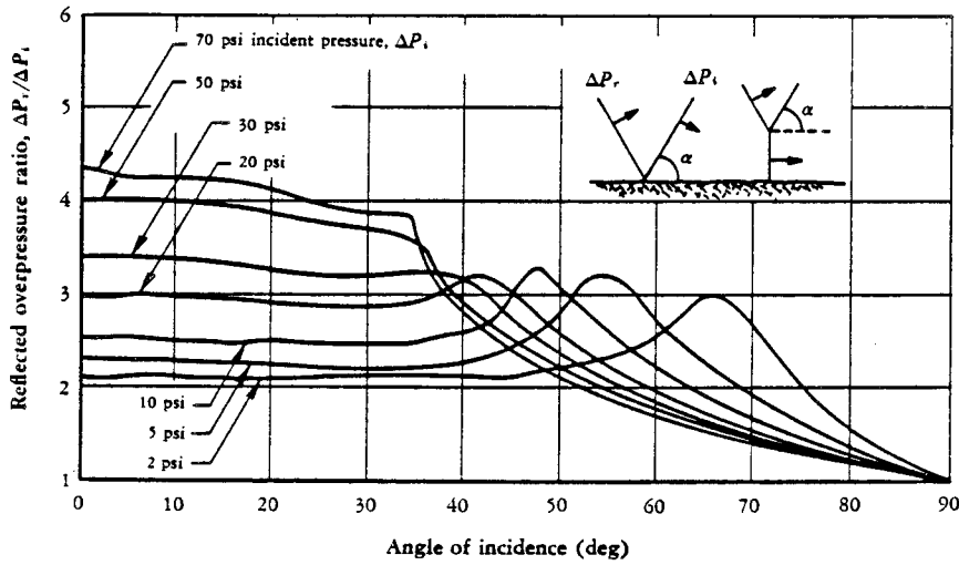
FIG. 33—Reflection Factors versus Incident Angle and Shock Strength
