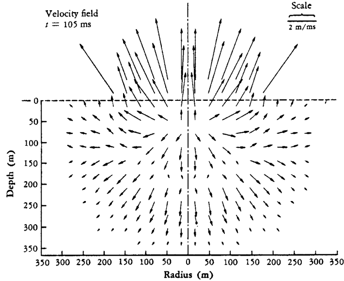
FIG. 19—Particle Velocities from Surface Burst ( t = 105 ms)
