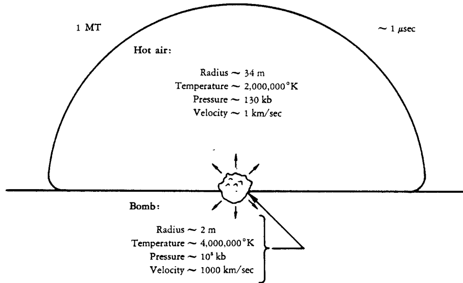
FIG. 13—Initial Conditions for Surface-burst Cratering Motion
