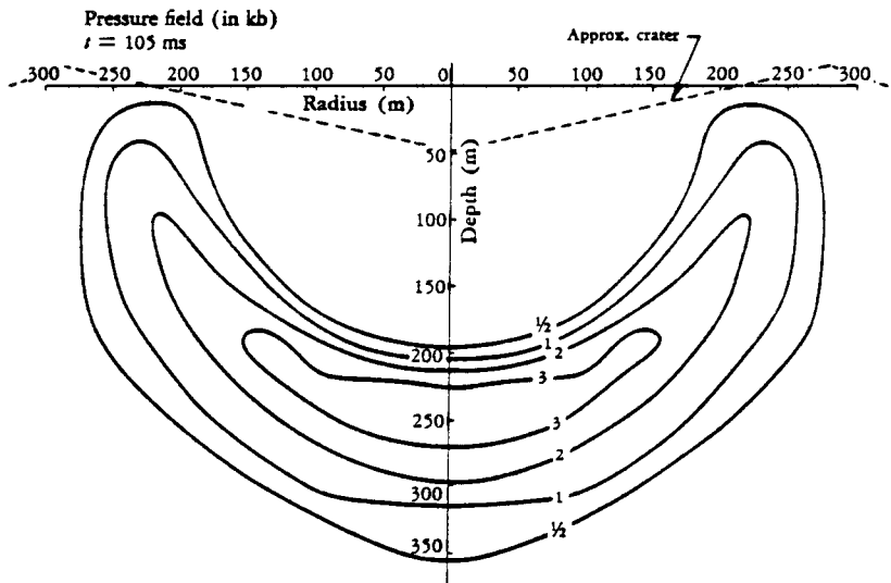
FIG. 18—Earth Pressure Contours from Surface Burst ( t = 105 \text{ ms} )
