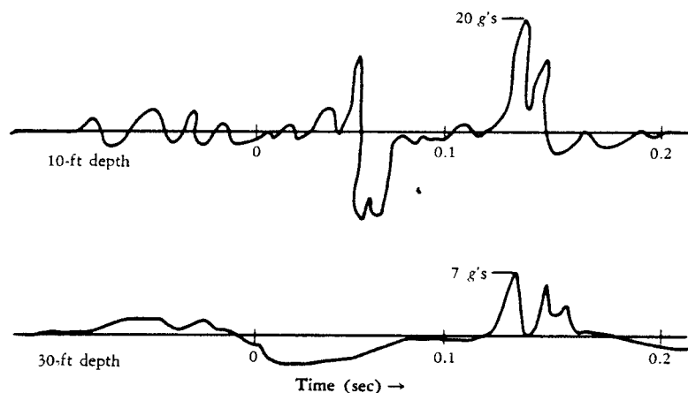
FIG. 42—Vertical Accelerations at Shallow Depths
