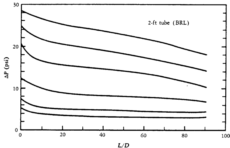
FIG. 39—Shock-tube Attenuation Data at Low Overpressure
