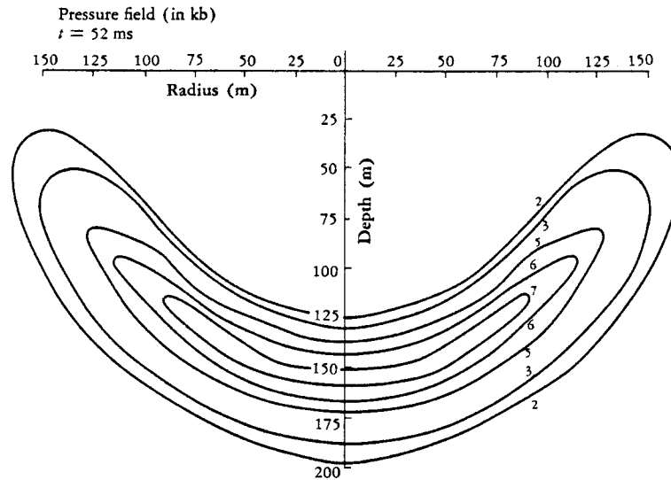
FIG. 16—Earth Pressure Contours from Surface Burst ( t = 52 ms)
