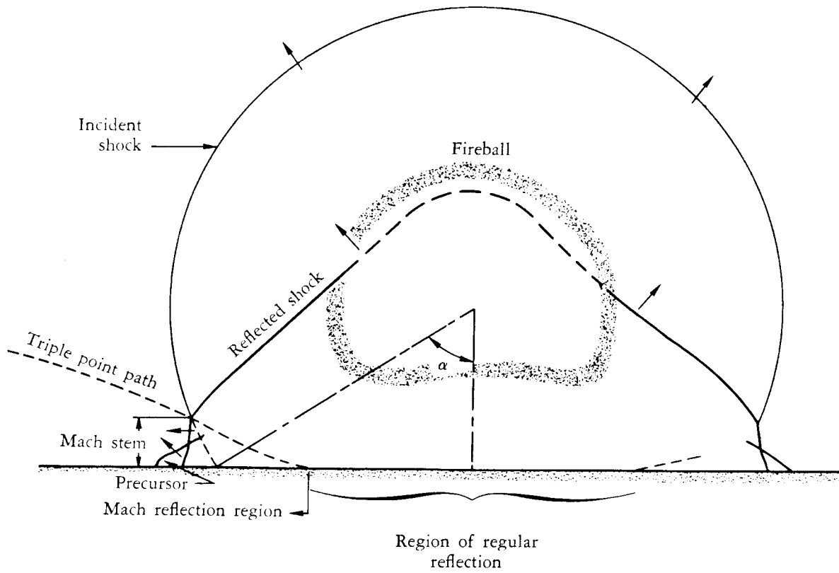
Fig.21 — Shock configurations (air burst)
