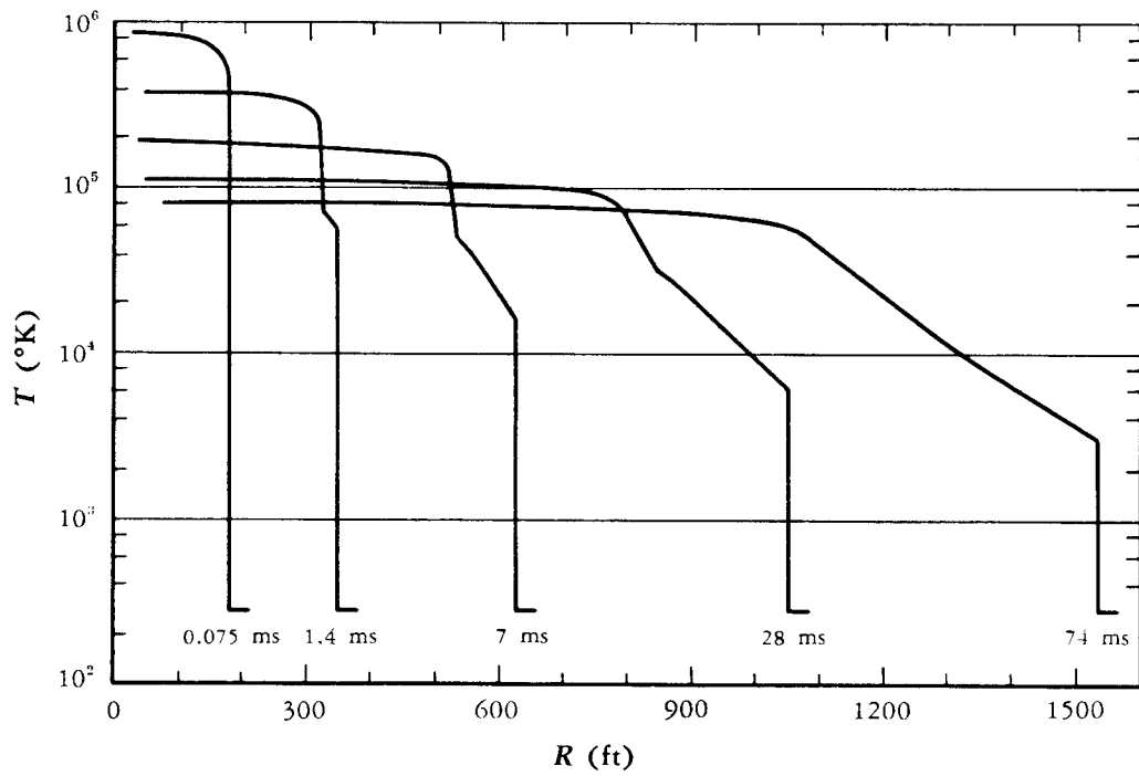
Fig.4—Fireball temperature versus radius at early times in the fireball history (1-MT surface burst)
