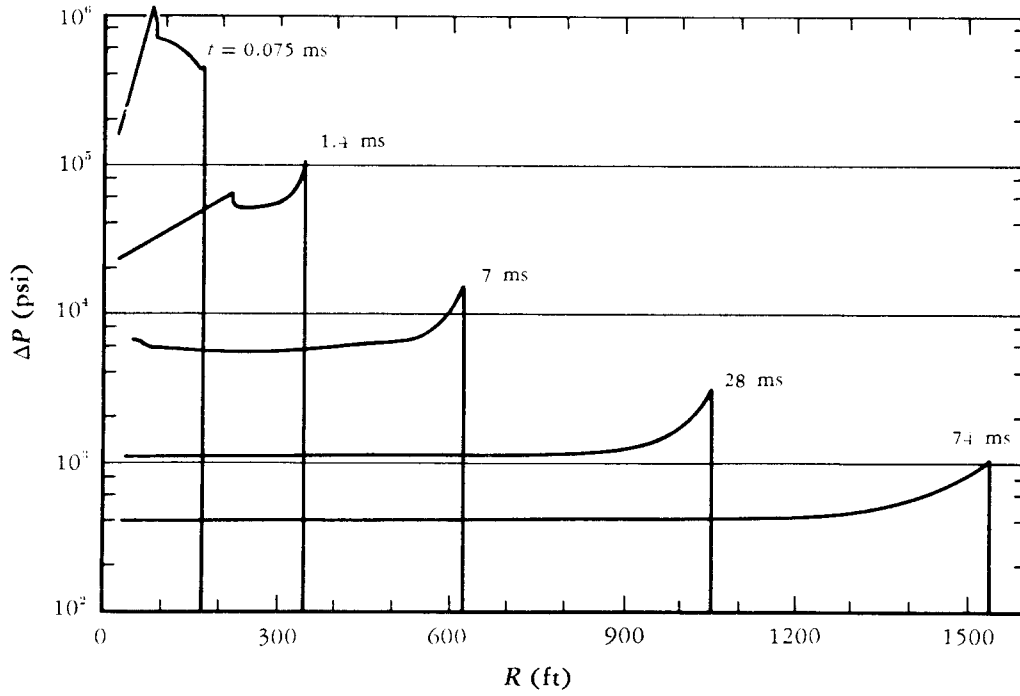
Fig.7—Overpressure versus range at early times in the shock-wave growth (1-MT surface burst)
