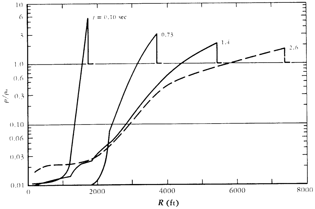
Fig.16—Late fireball densities (1-MT surface burst)
