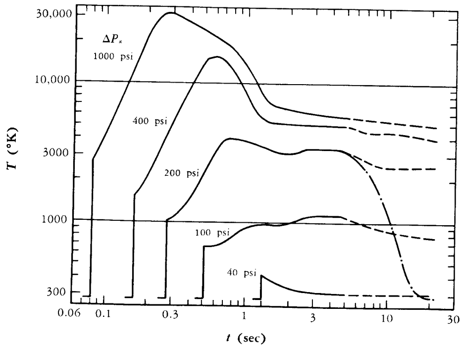
Fig.18—Temperature versus time at high peak overpressures (1-MT surface burst)
