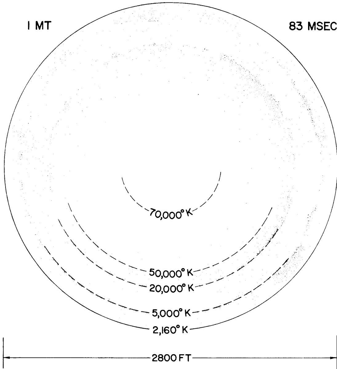
Fig. 14—Fireball size and temperature at a time near minimum light intensity
