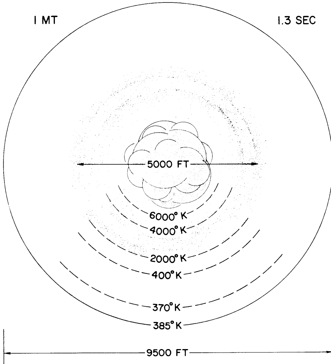
Fig. 17—Late shock and fireball size and temperature
