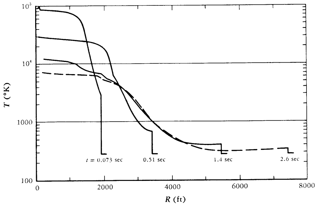
Fig.15—Late fireball temperature versus radius
