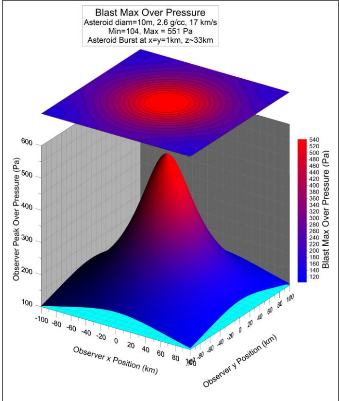
Figure 49 – Shock wave max pressure vs observer position on a 200x200km ground grid for a 10m diameter asteroid/fragment at 17km/s and density 2.6g/cc.
