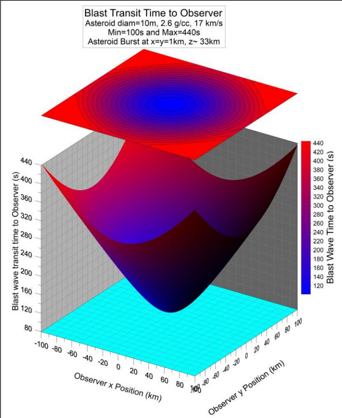
Figure 50 – Shock wave transit time from burst to observer vs observer position on a 200x200km ground grid for a 10m diameter asteroid/fragment at 17km/s and density 2.6g/cc.
