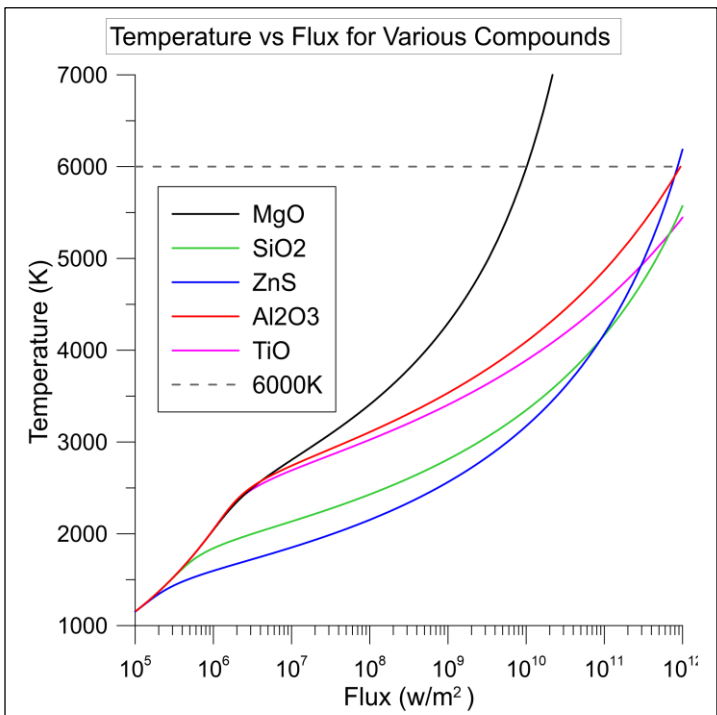
Figure 143 – Bolide ablation temperature vs atmospheric ram flux for various high temperature refractory compounds.
