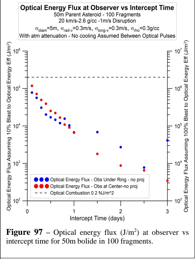
Figure 96 – Blast wave peak pressure vs arrival time for 5 hour intercept of 50m bolide in 100 fragments.
