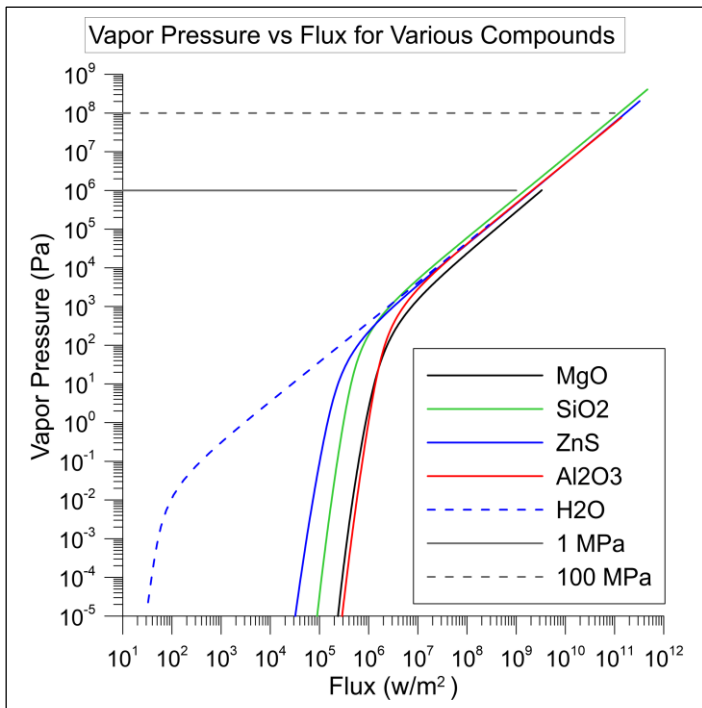
Figure 144 – Bolide ablation vapor pressure vs atmospheric ram flux for various compounds including high temperature refractory compounds and low temp (H 2 O).
